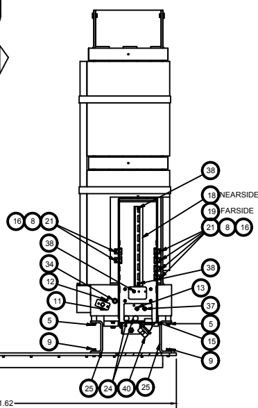
SECTION F-F SCALE 1 / 8
